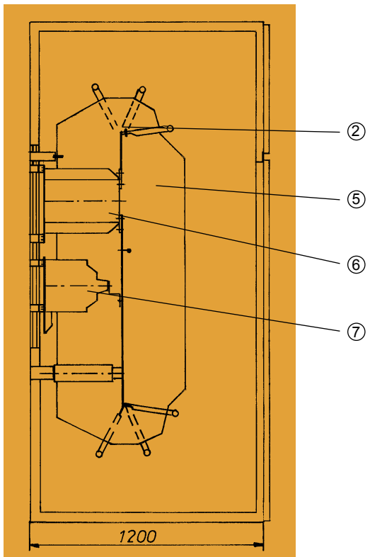
Fig. 9: 36 kV Measuring panel
