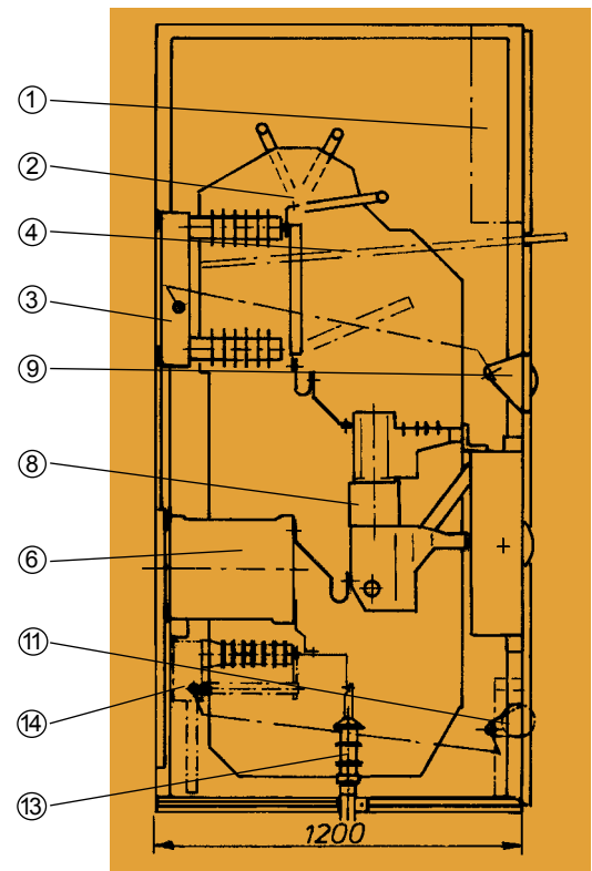
Fig. 10: 36 kV Switch panel with circuit-breaker V 620 KUF
