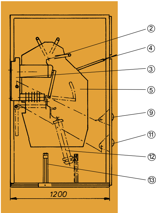
Fig. 2: 36 kV Cable panel with switch-disconnector H 29 EA
