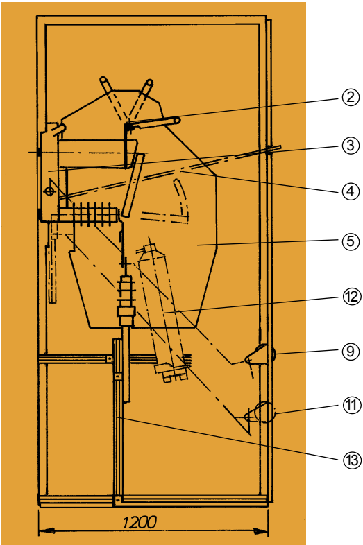
Fig. 7: 36 kV Cable panel with switch-disconnector H 29 EA
