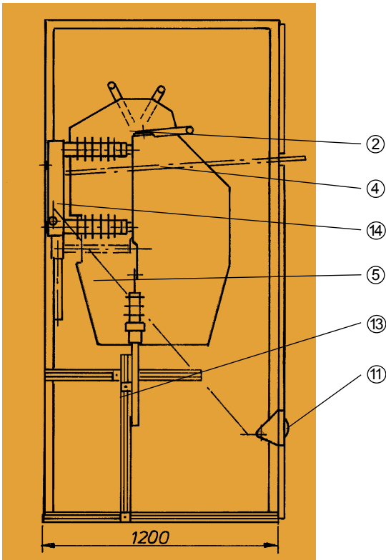
Fig. 11: 36 kV Cable riser panel
