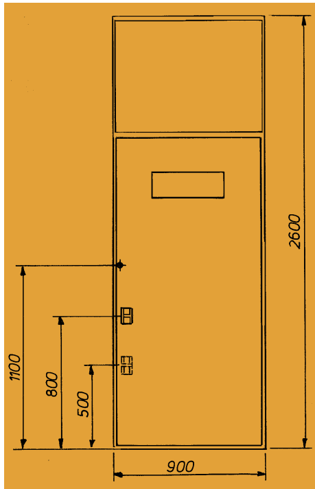
Fig. 5: 36 kV Switch panel with Switch-disconnector H 29
