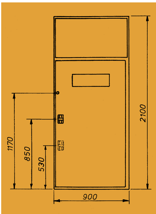
Fig. 1: 36 kV Switch panel
