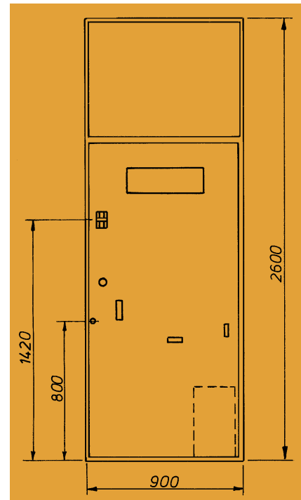
Fig. 6: 36 kV Switch panel with circuit breaker
